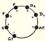
EBC91-6AV6
