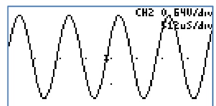
Figure 14: Slope trigger
