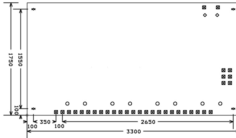
Figure 4: Xminilab dimensions
